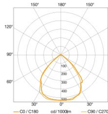
Light distribution curve for RS PRO DL LED 14W — C0 / C180 cd/1000lm — C90 / C270
