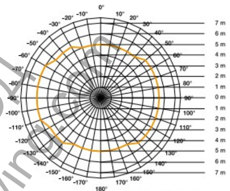
RS PRO DL LED 14 W detection zone Mounting height 2.8 m orange = radial walking direction
